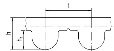
Figure 1.4.9: HTD profile
